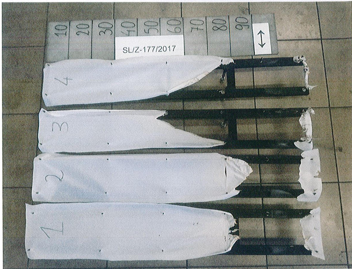
Figure 3. Appearance of the sample 2 after the test – cross direction
