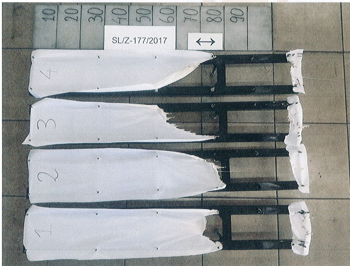
Figure 2. Appearance of the sample 1 after the test - lenght direction
